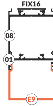
Variante 15 - Deckenversion FIX16-08-01-E9 variant 15 - ceiling FIX16-08-01-E9
