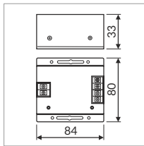
LED Controller warmweiß-kaltweiß 2 Kanäle LED receiver warm-cold 2 channel 12V/24VDC; 144W/288W
