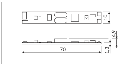
LED Controller Basisversion 1 Kanal LED receiver basic 1 channel 12-24 V; 60-100 W
