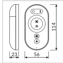
LED RGB Fernbedienung LED remote controller RGB
