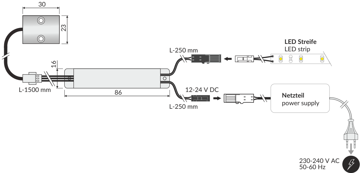
LED Türschalter berührungslos LED switch door operated sensor 12-24 V; 30 W
