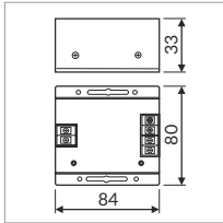
LED RGB Controller 3 Kanäle LED receiver RGB 3 channel 12V/24VDC; 216W/432W
