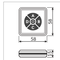
LED Fernbedienung Basisversion 4 Kanäle LED remote controller basic 4 channel
