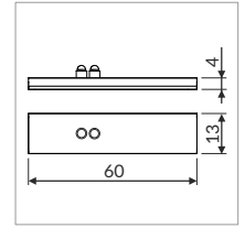
LED Schalter SU/GR/CO berührunglos dimmbar LED switch SU/GR/CO touchless dimmable 12-24 V; 60-100 W
